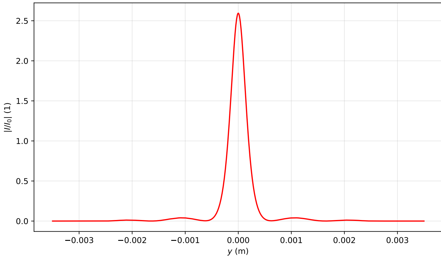
Intensity profile I(x=0, y, z=0.796)/I_0 , P_{in}=1.0P_{cr} , artificial time
